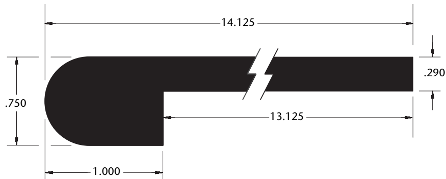
EXCLUSIVE ONE STEP® STAIR TREAD
